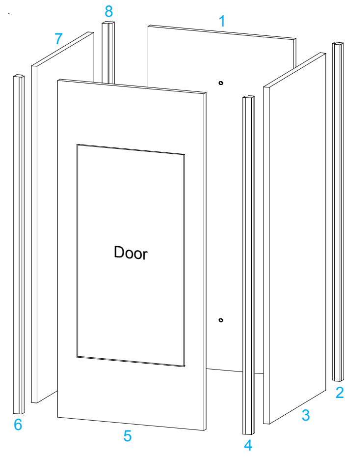
Pedestal Base Assembly
